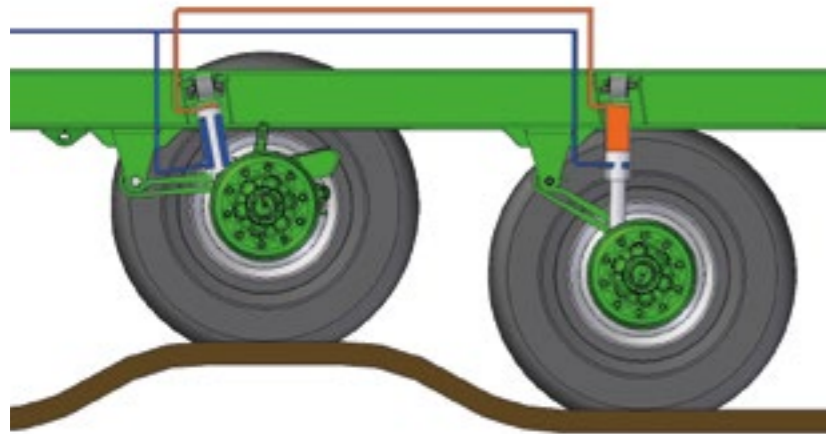
Teli hydraulisella rungolla
