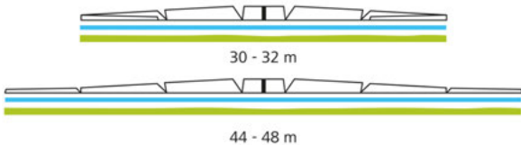
BoomControl – 7-part with reduced working width 30 m
