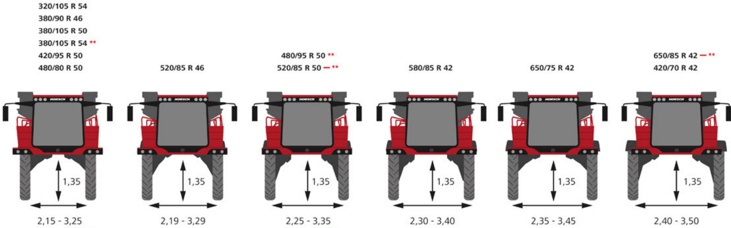
Leeb VT flange size adjustment 2.22 m - 3.32 m (**with L12 boom)
